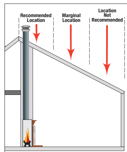
Fig. 3. The chimney should penetrate a vaulted ceiling at or near its highest point.
